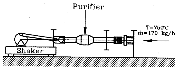
Figure 1. Test Bench Schematic
