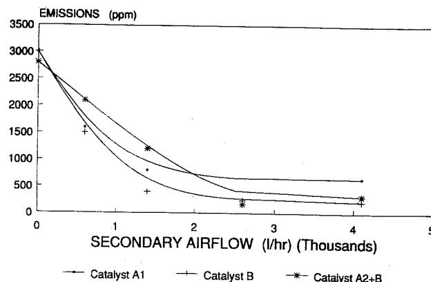
Fig. 18 HC Emissions Versus Secondary Airflow Load = 3kW, Baseline = 2300 ppm
