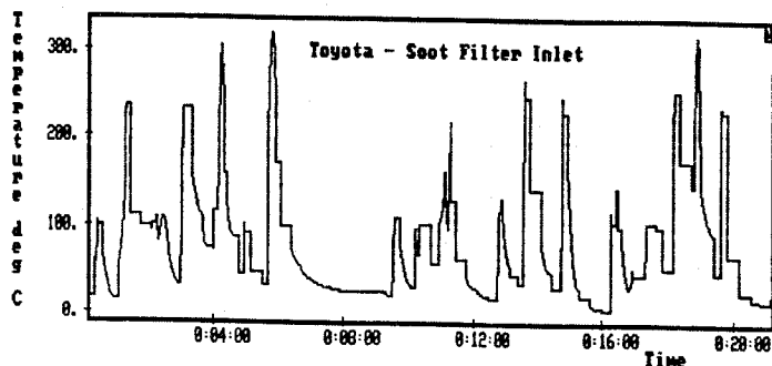
Fig.3 Toyota Land Cruiser exhaust gas temperature recording
